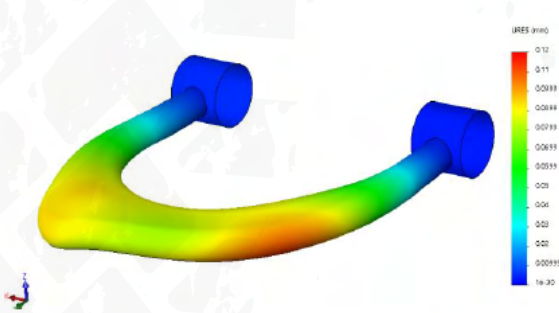
Max Displacement = 0.12 mm
