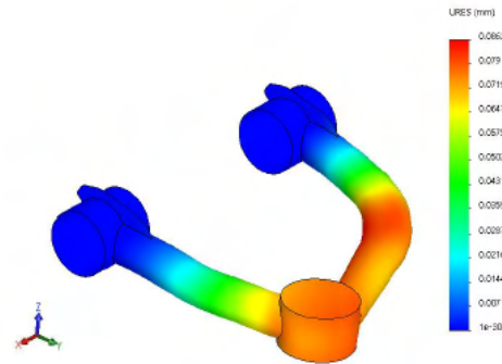
Max Displacement = 0.09 mm
